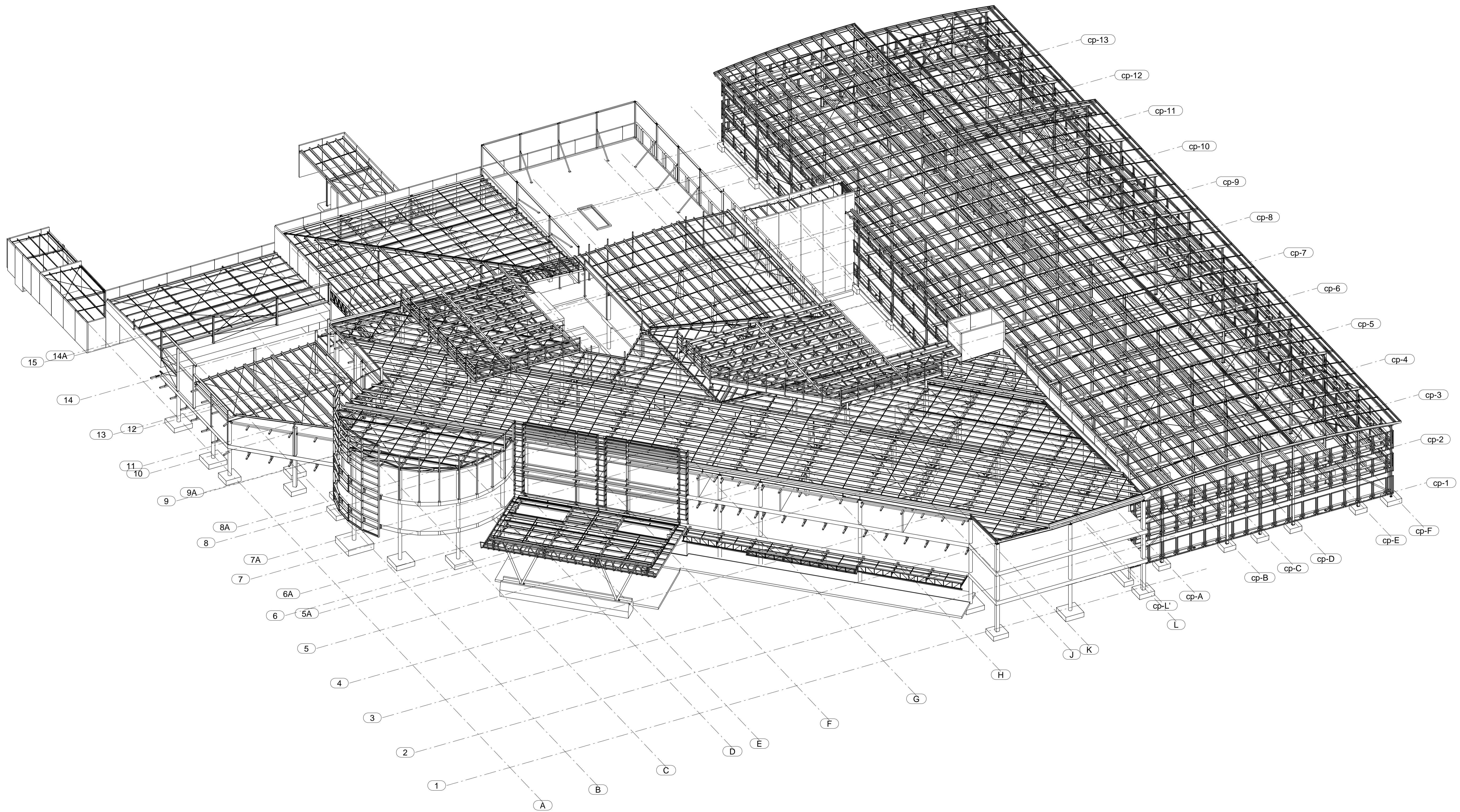
MAIN BUILDING & CARPARK - PERSPECTIVE VIEW
