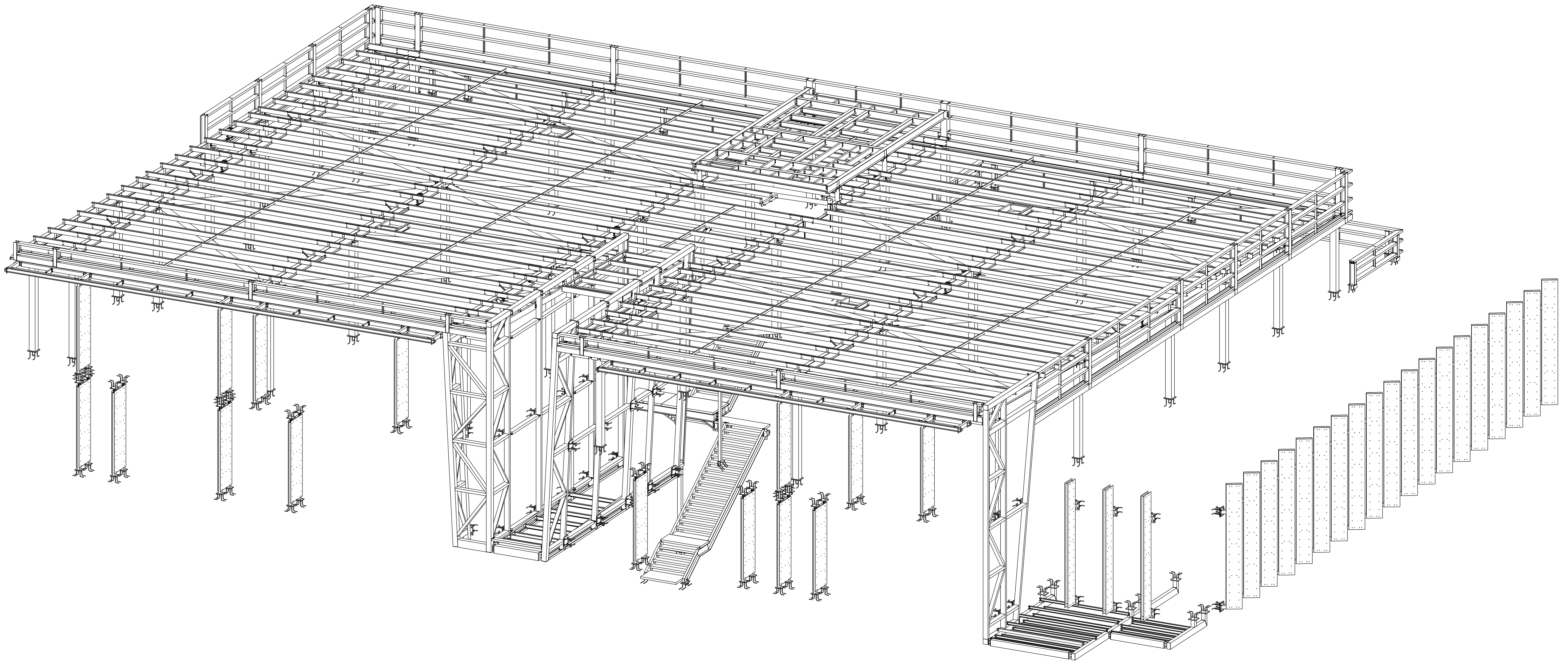
STEELWORK PERSPECTIVE VIEW
