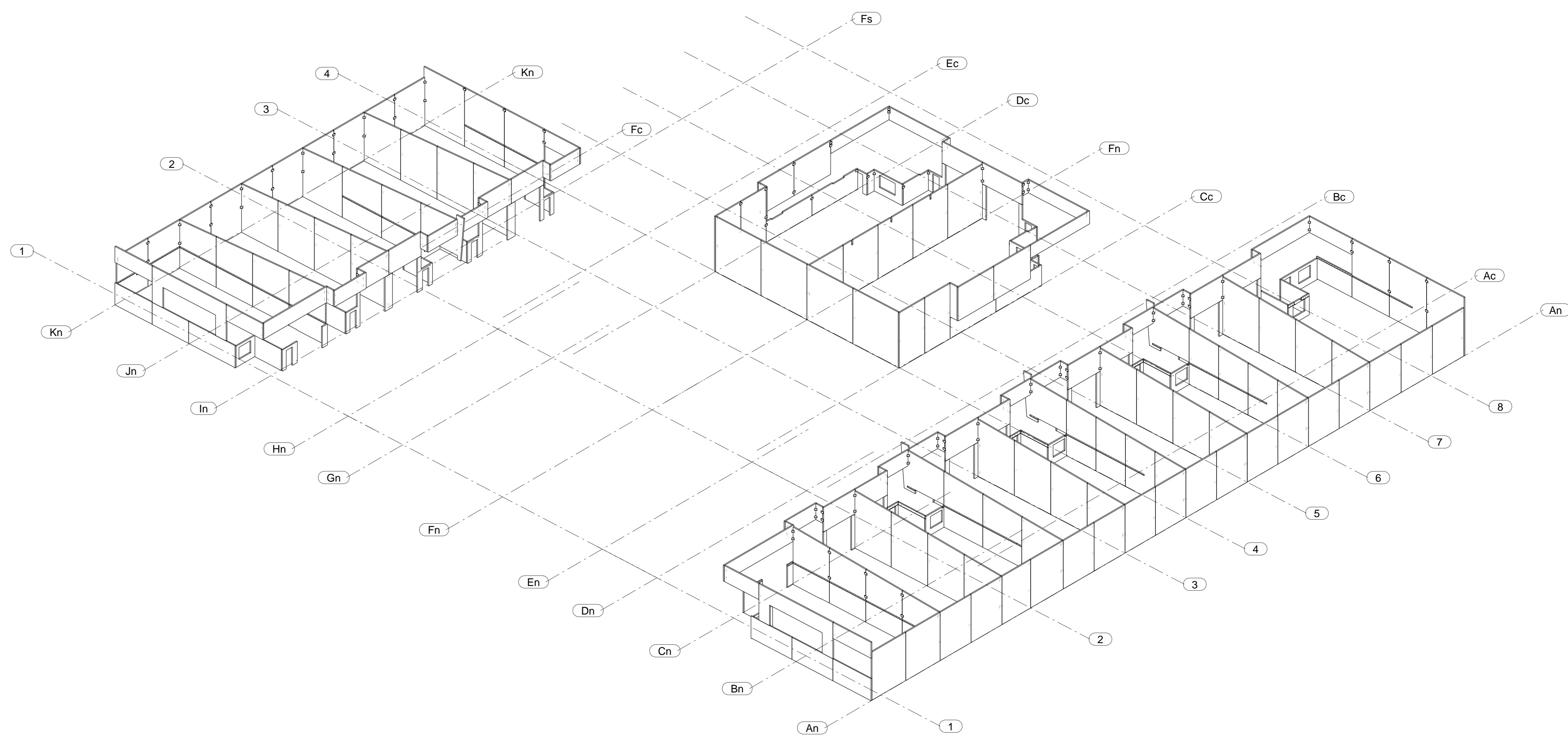
3D VIEW - FIRST FLOOR RL+97.08 RC BEAMS AND SLABS NOT SHOWN
