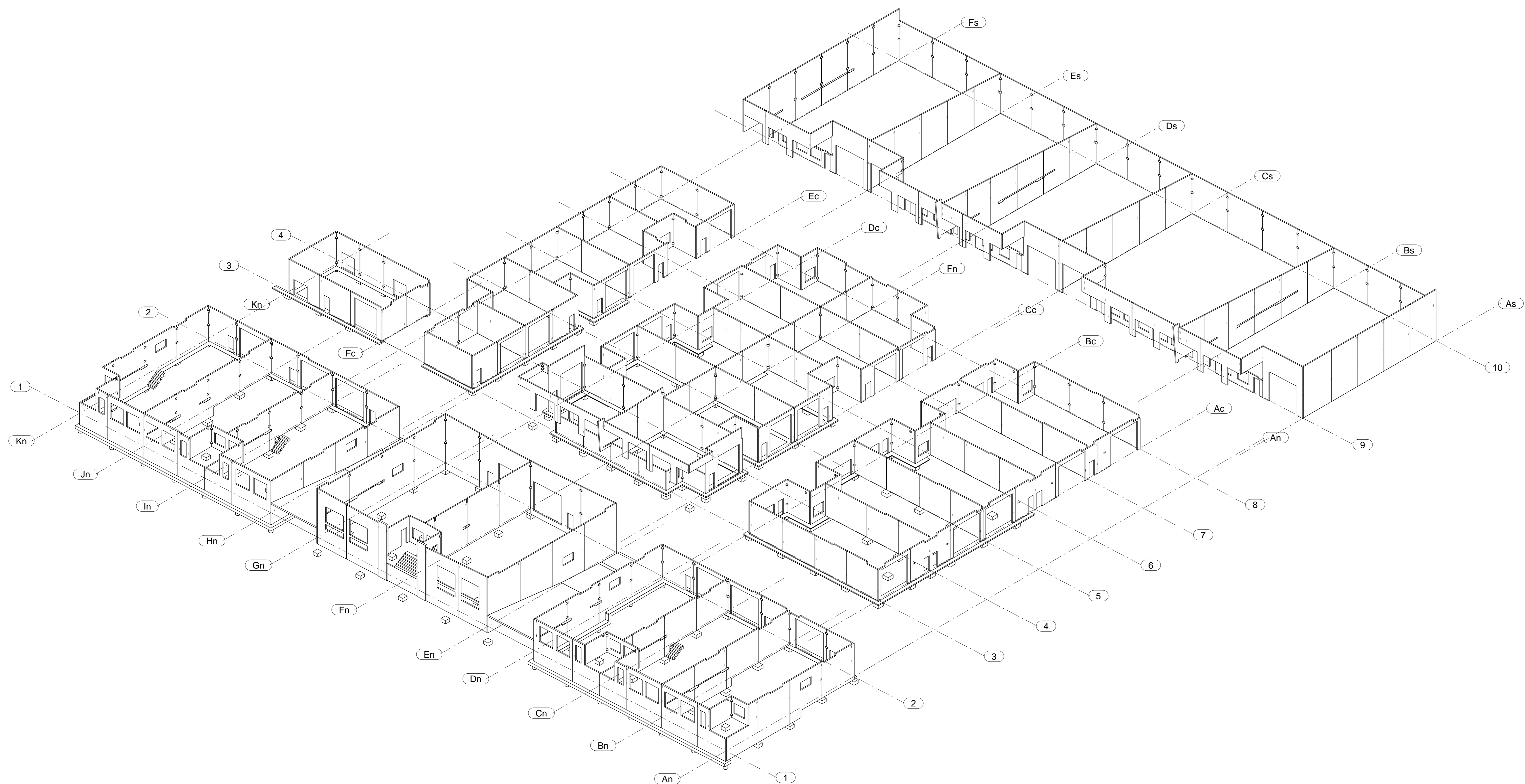
3D VIEW - GROUND FLOOR RL+91.68 RC BEAMS AND SLABS NOT SHOWN
