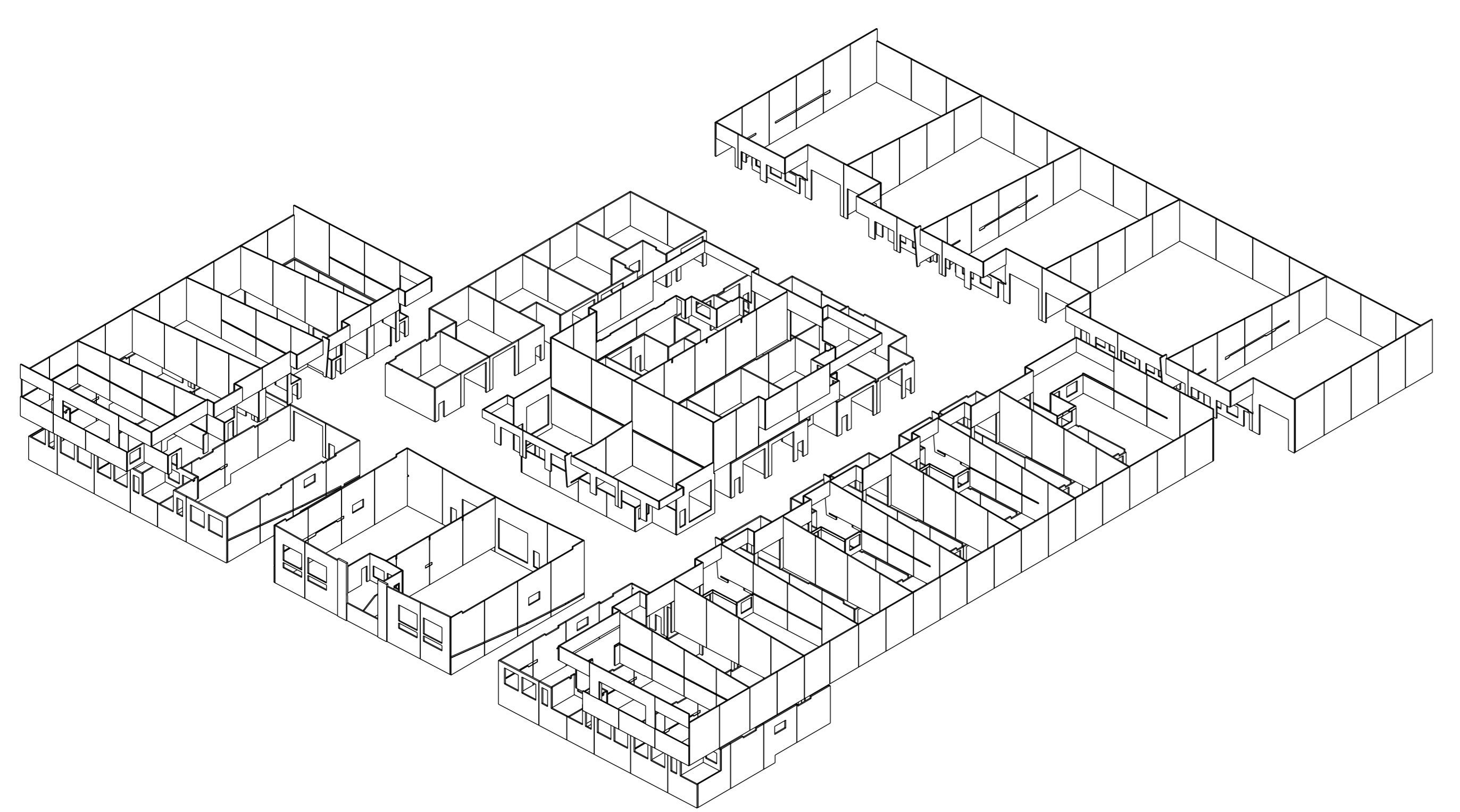
ALL BLOCKS - PANELS ONLY
