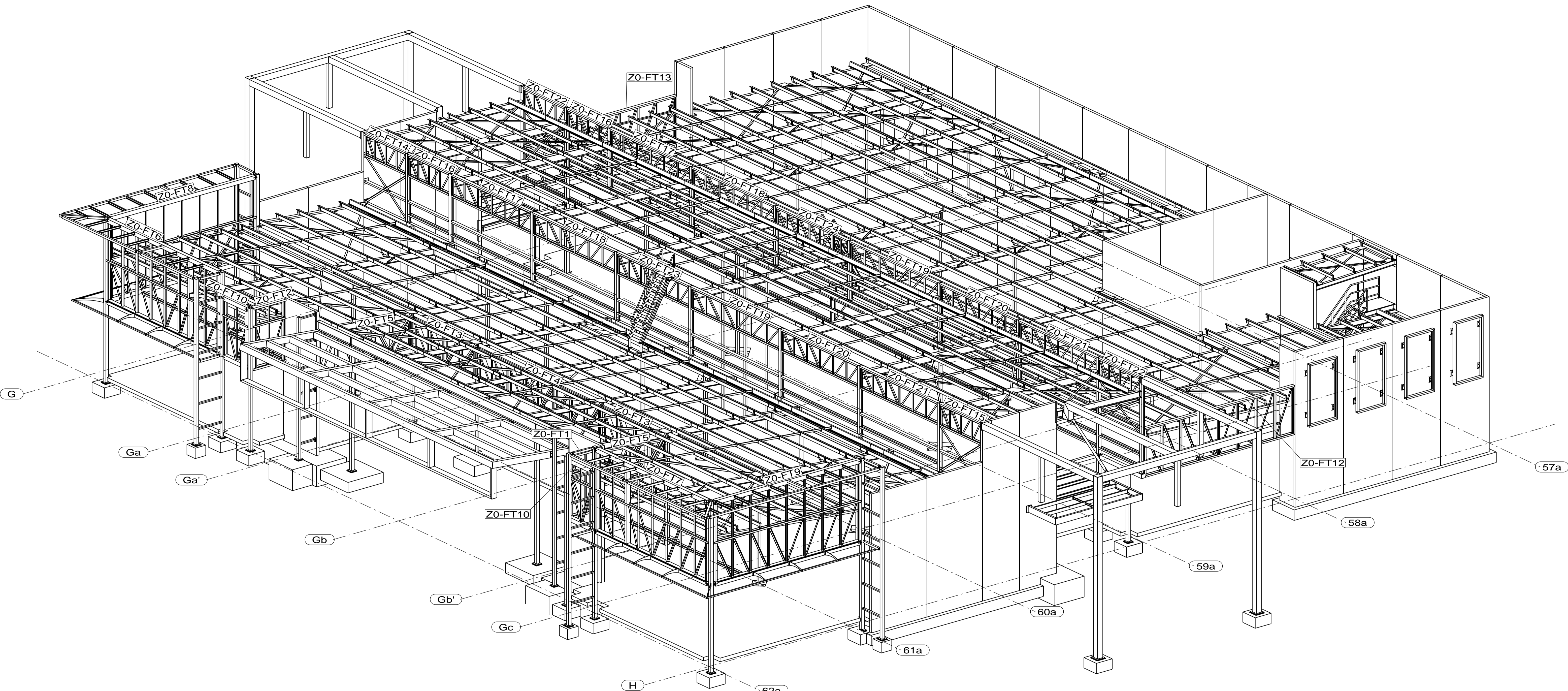
ZONE 10 (FOOD COURT) - PERSPECTIVE VIEW
